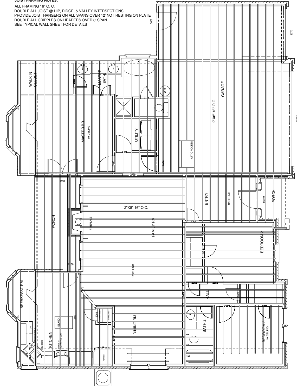
CEILING FRAMING PLAN
